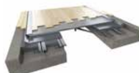
426/427/428 Series - Centering Bar, Interior Floor
