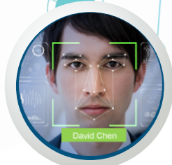
Face Recognition
